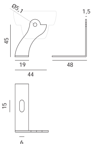
Staffa orientabile Adjustable bracket
